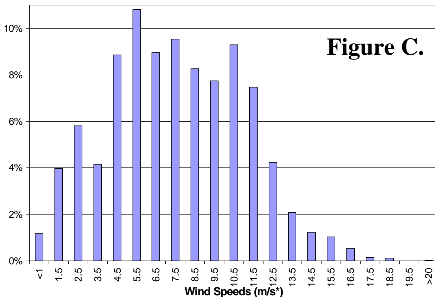
Frequency Distribution of Wind Speeds at 70 meters
